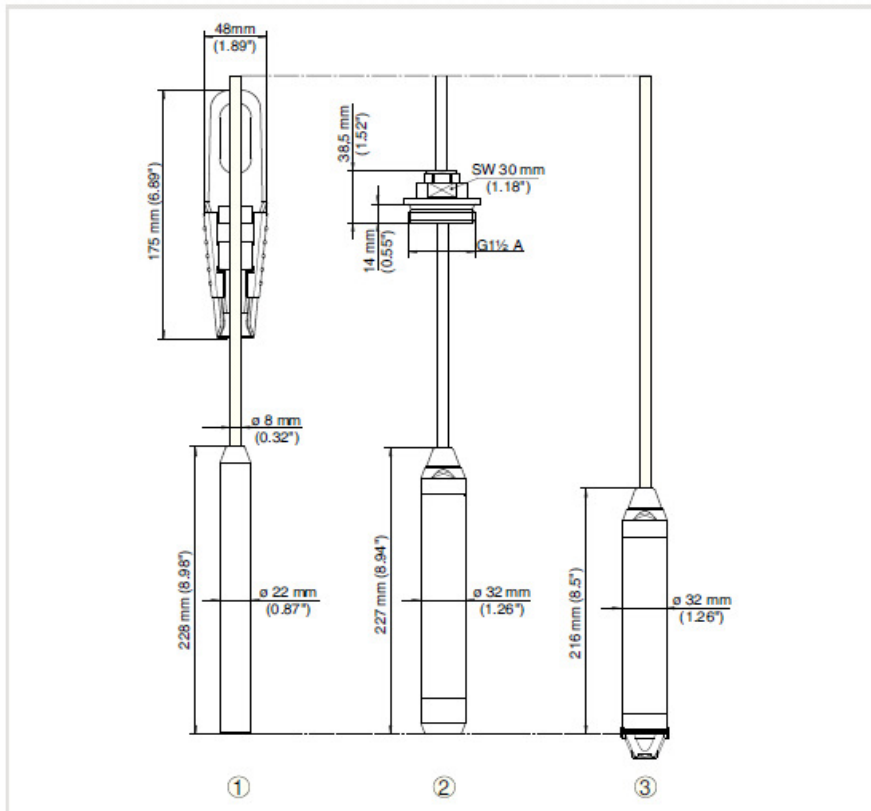
Dimensions VEGAWELL 52
